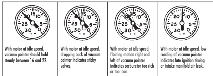
FIGURE 5: VACUUM GAUGE READINGS
