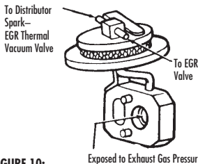
FIGURE 10: EXHAUST BACKPRESSURE TRANSDUCER VALVE
